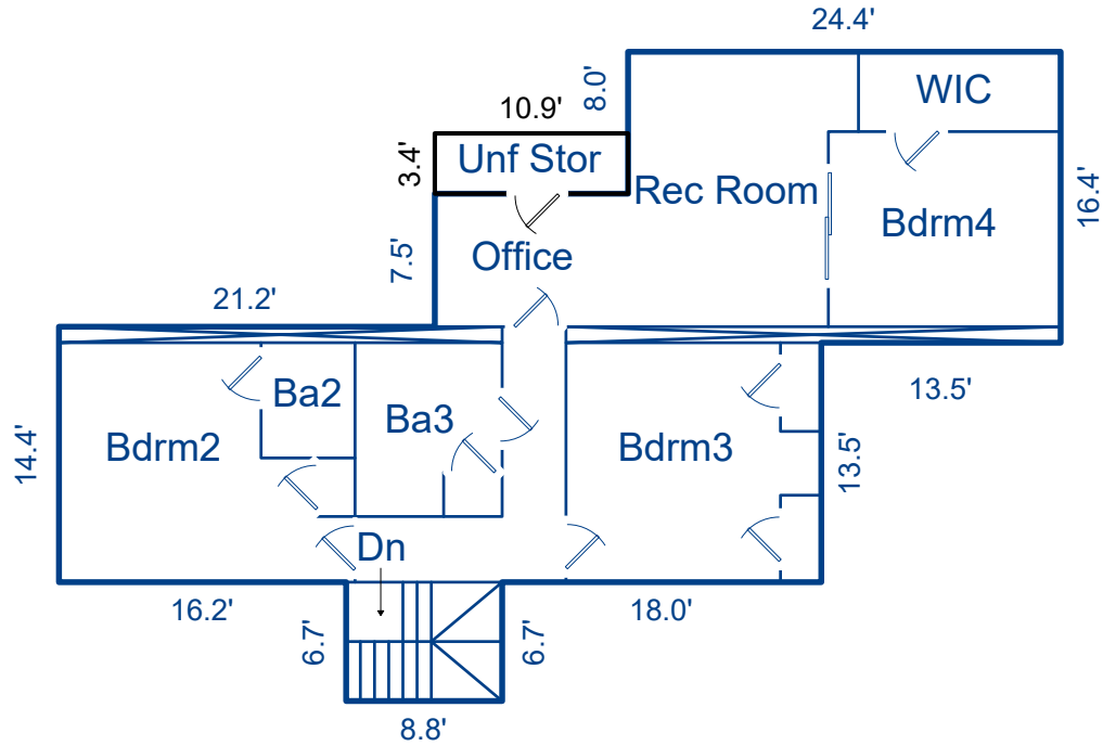
Second Floor 1150.3 sf
